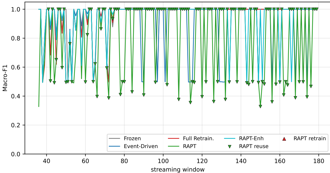
UGR'16 — per-window macro-F1 (seed 42)
